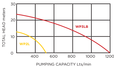
PERFORMANCE CURVE
