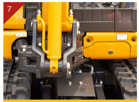
Offset boom - for increased visibility and boom rotation
